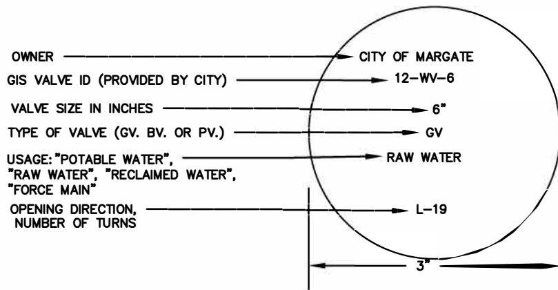
VALVE IDENTIFICATION MARKERS (TAG)
