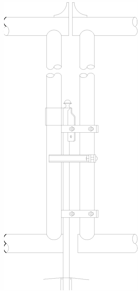
ELEVATION OF LOCKING DEVICE FOR DOUBLE GATES
