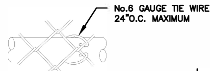
WIRE TIES FOR BRACE RAIL
