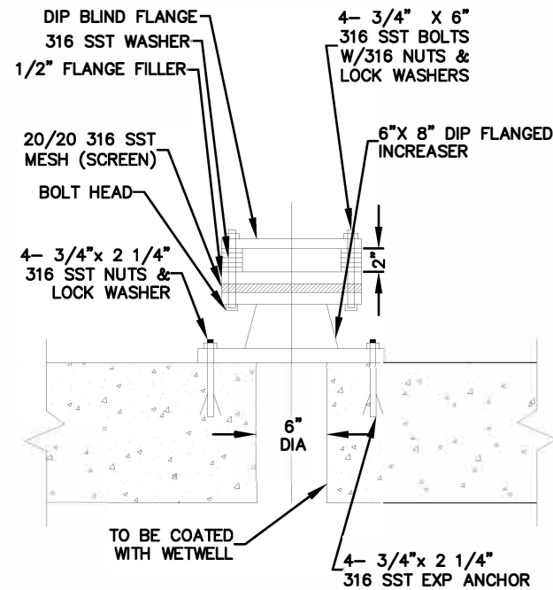
6" WETWELL VENT DETAIL NTS
